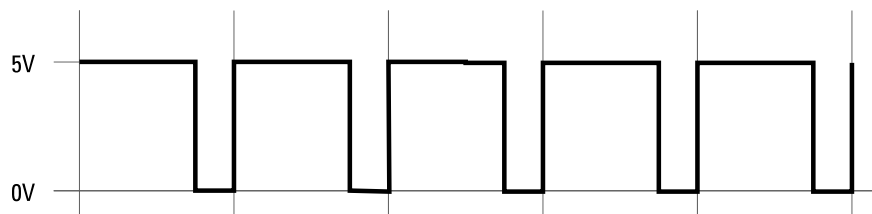
Figure 5-4: Using pulse-width modulation to change how long a digital pin is on or off. The vertical lines represent regular time intervals, usually 700 cycles per second.
