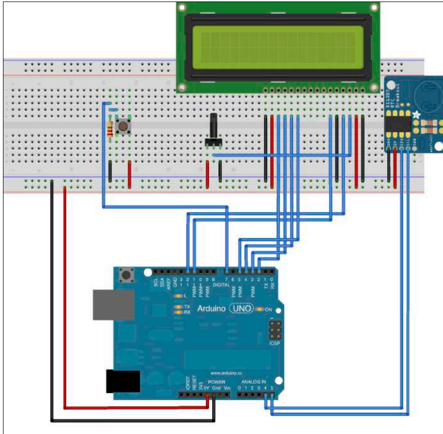
Figure 7-6: Parts place- ment for the alarm hours pushbutton.
