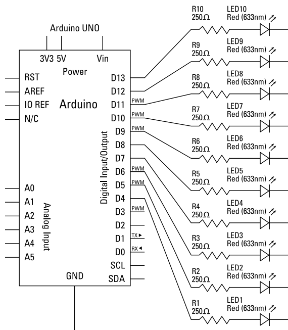
Figure 4-4: Schematic diagram of the all- seeing eye.
