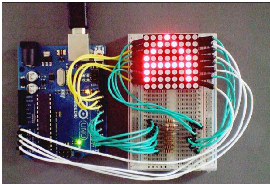
Figure 6-6: Displaying scrolling text.
