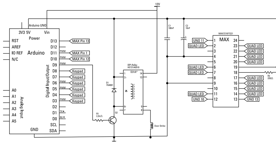
Figure 8-4: Schematic diagram of the keypad entry system.
