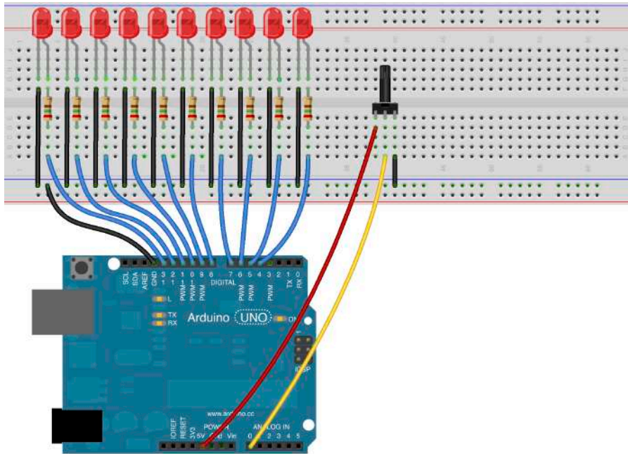
Figure 4-5: Using a potentiometer to create the simplest analog input circuit.
