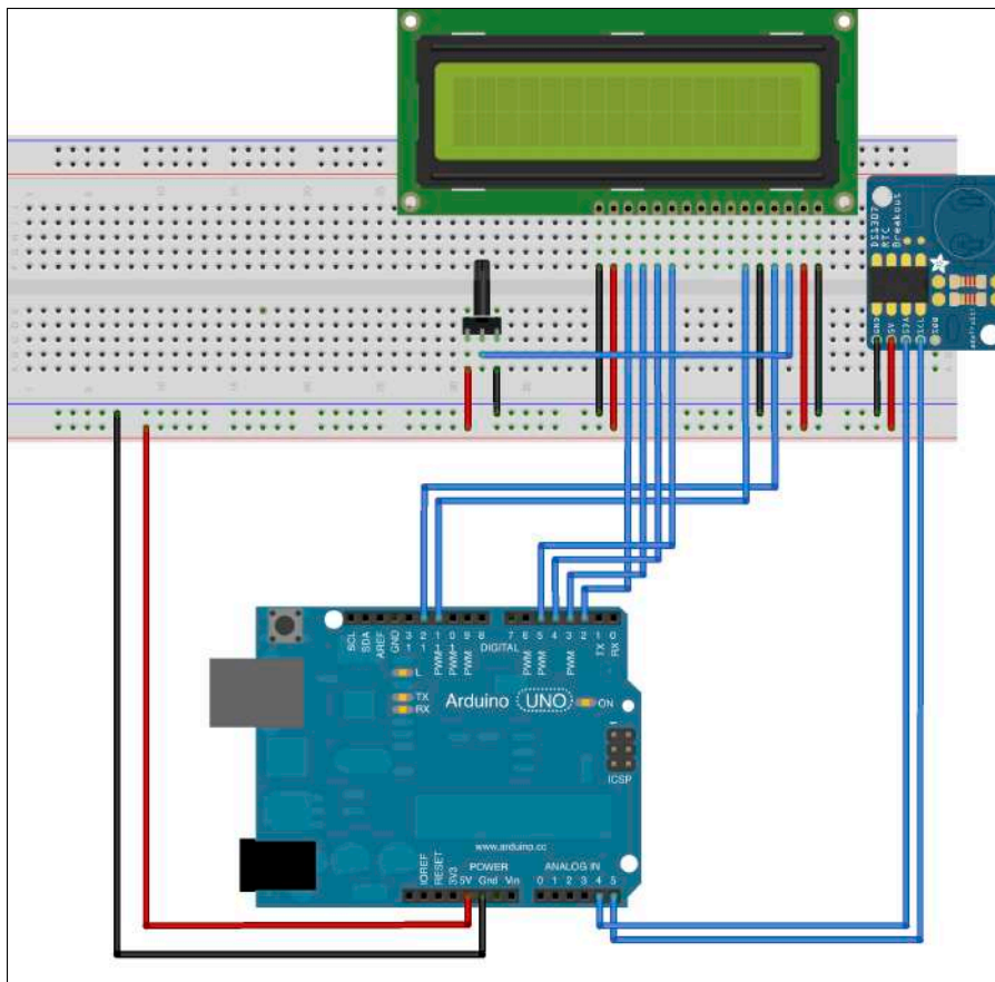
Figure 7-5: Parts place- ment for adding the 16 x 2 LCD display.
